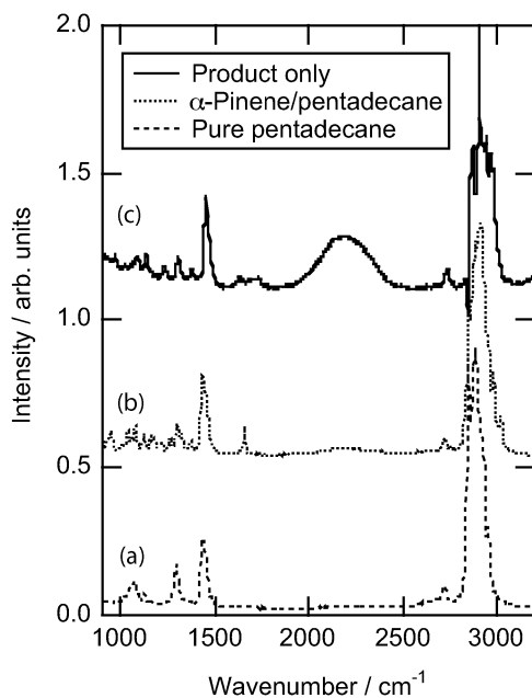
Fig. 4 Raman spectra (intensity as a function of the relative wavenumber) of (a) a pure pentadecane droplet, (b) a droplet of \alpha -pinene and pentadecane before reaction with ozone, mole fraction of \alpha -pinene is \sim 0.66 , and (c) the Raman spectrum obtained after reaction with ozone, from which the reactants ( \alpha -pinene and pentadecane) have been subtracted. Spectrum (c) has several product peaks in the region 1600\text{--}1800\text{ cm}^{-1} characteristic of C=O stretches. The peaks characteristic of the carbon–carbon double bond stretches in \alpha -pinene can be found in spectrum (b) at 1640\text{ cm}^{-1} , and the two peaks between 3000 and 3100\text{ cm}^{-1} are gone in spectrum (c). The broad feature centered on 2200\text{ cm}^{-1} in spectrum (c) is stray light used to image the droplet/particle and can be removed by subtraction of background signal. The sharp feature at 2850\text{ cm}^{-1} in spectrum (c) is a morphological Raman resonance, and is included to demonstrate its occurrence in some spectra. The particle studied had 4.7\text{ }\mu\text{m} radius, the relative humidity was 10% and [\text{O}_3] was at 0.4\text{ ppm} .
